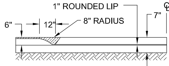
SECTION AT GUTTER LINE
