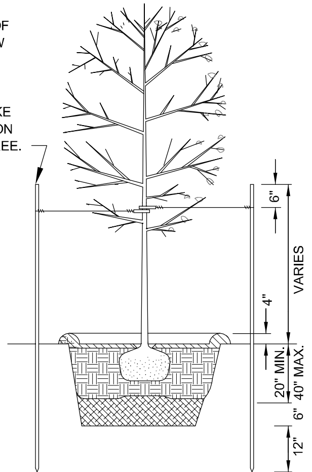
TREE STAKING - LEVEL GROUND
