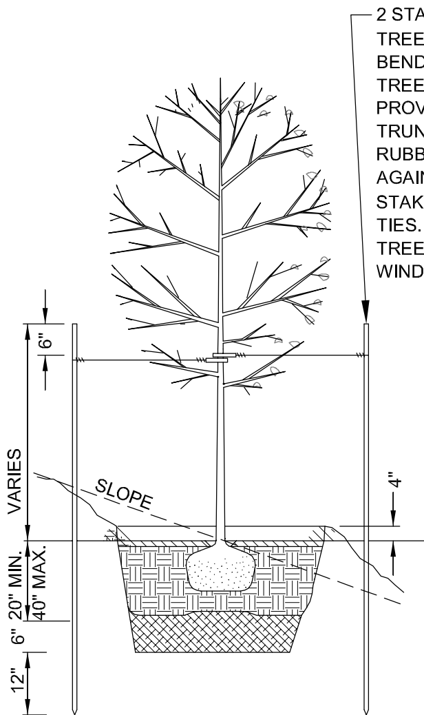
TREE STAKING - SLOPES
