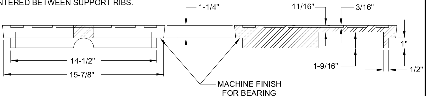
SIDE VIEW
