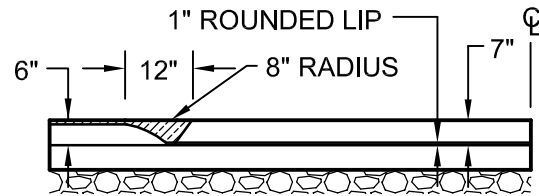
SECTION AT GUTTER LINE
