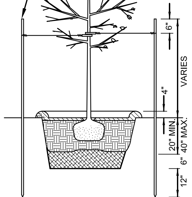
TREE STAKING - LEVEL GROUND
