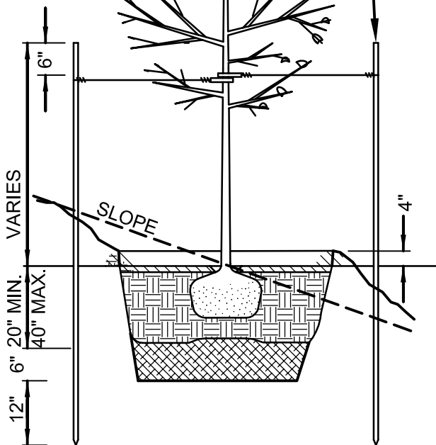
TREE STAKING - SLOPES
