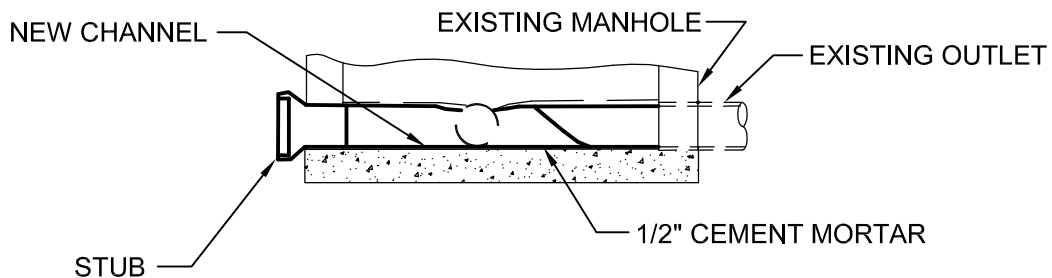
SECTION B-B
