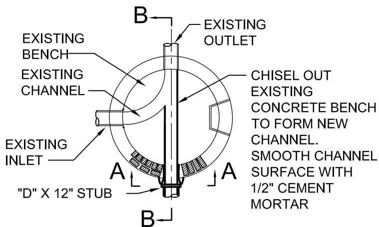
BASE PLAN OF BRICK MANHOLE
