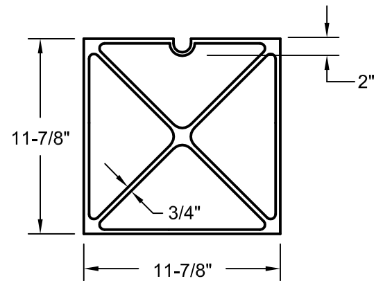
BOTTOM VIEW: COVER
