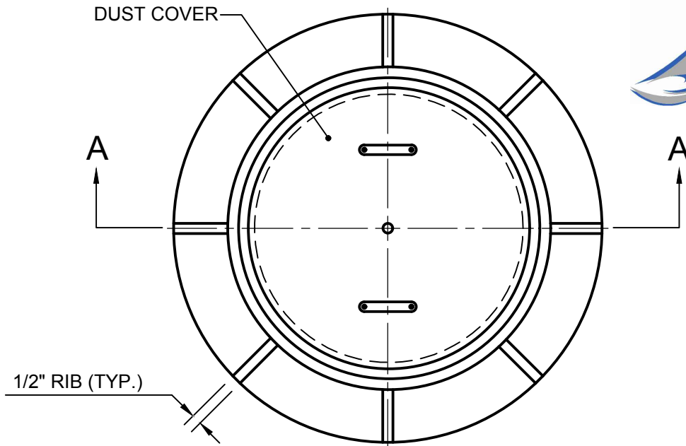
PLAN: CASTING
