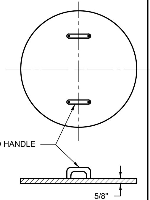
DUST COVER
