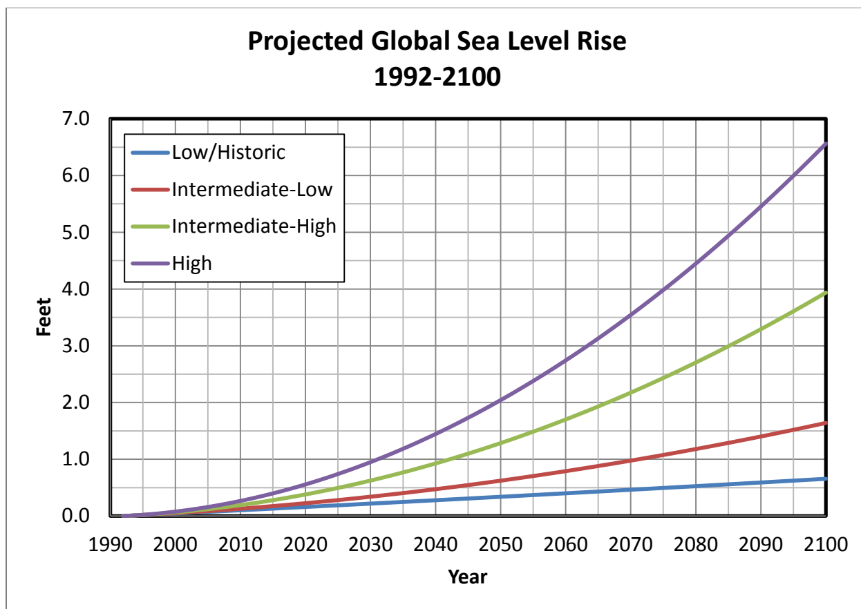
FIGURE 1: PROJECTED GLOBAL SEA LEVEL RISE, 1992-2100
