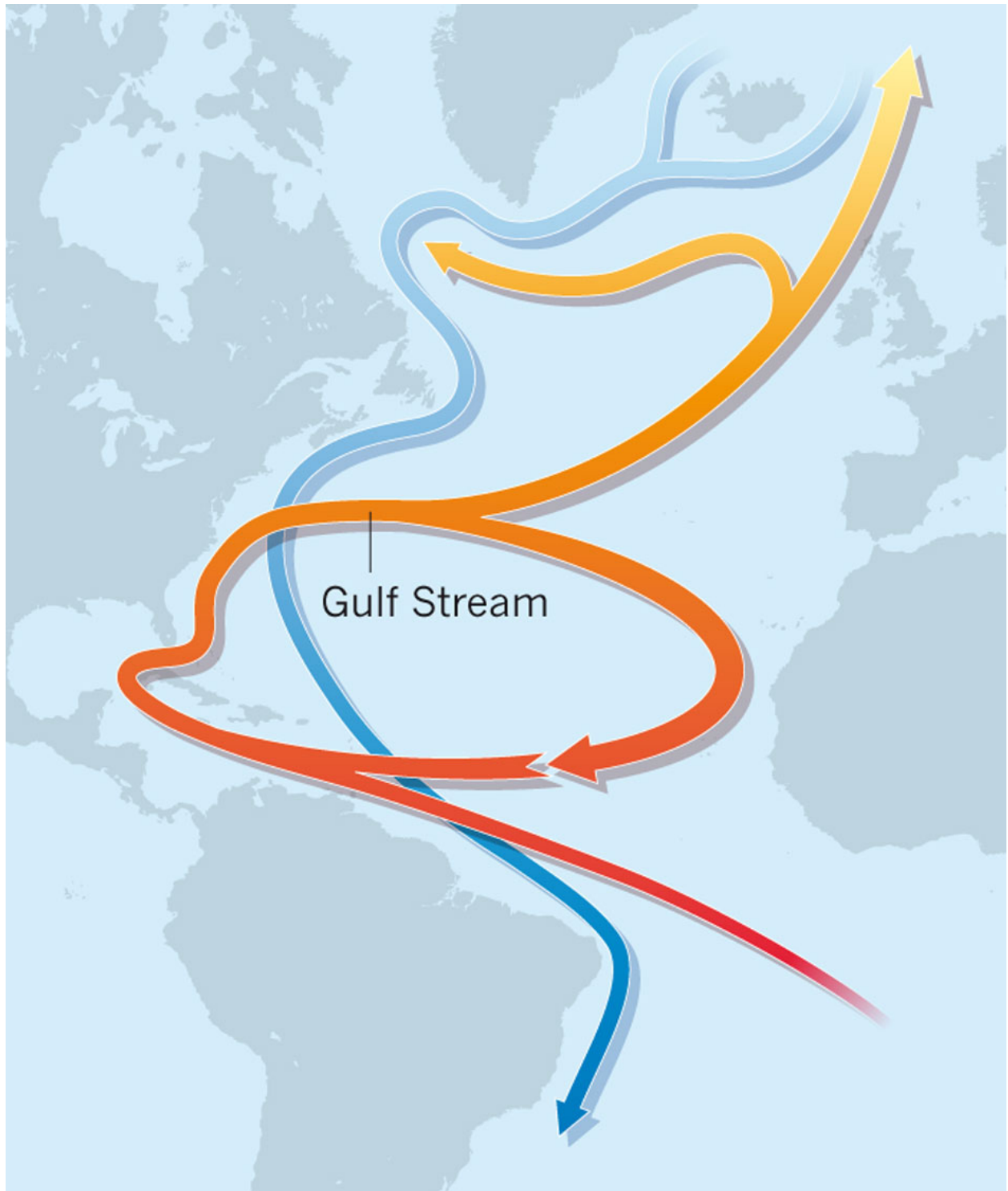
FIGURE 2: THE ATLANTIC MERIDIONAL OVERTURNING CIRCULATION (MAROTZKE 2012)
