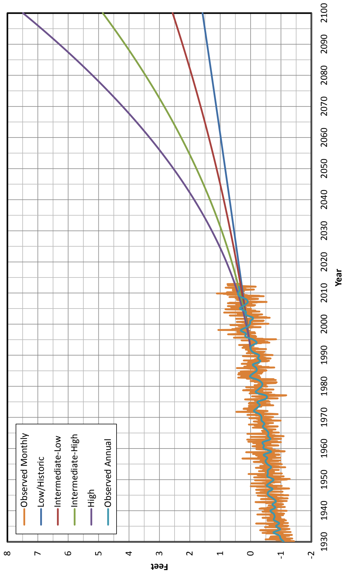
FIGURE 3: OBSERVED AND PROJECTED RELATIVE SEA LEVEL CHANGE, NORFOLK, VIRGINIA, 1930-2100
