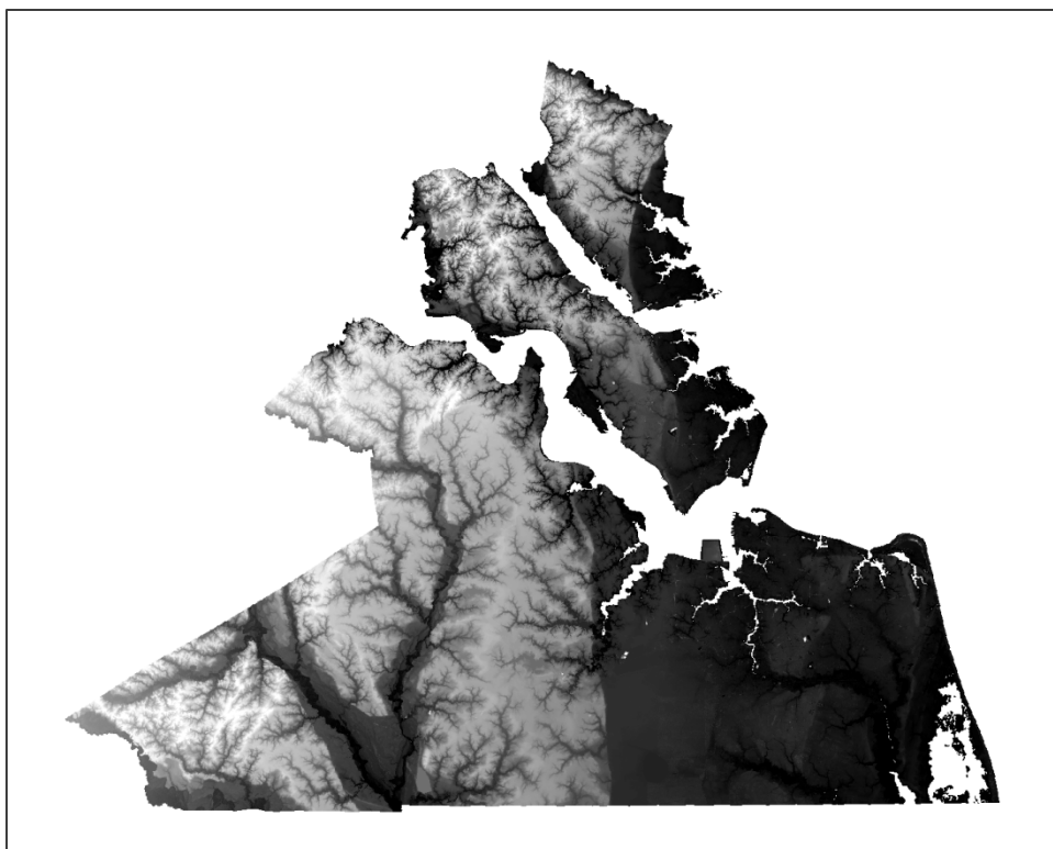
The original seamless regional Digital Elevation Model. Lighter areas are higher in elevation.
