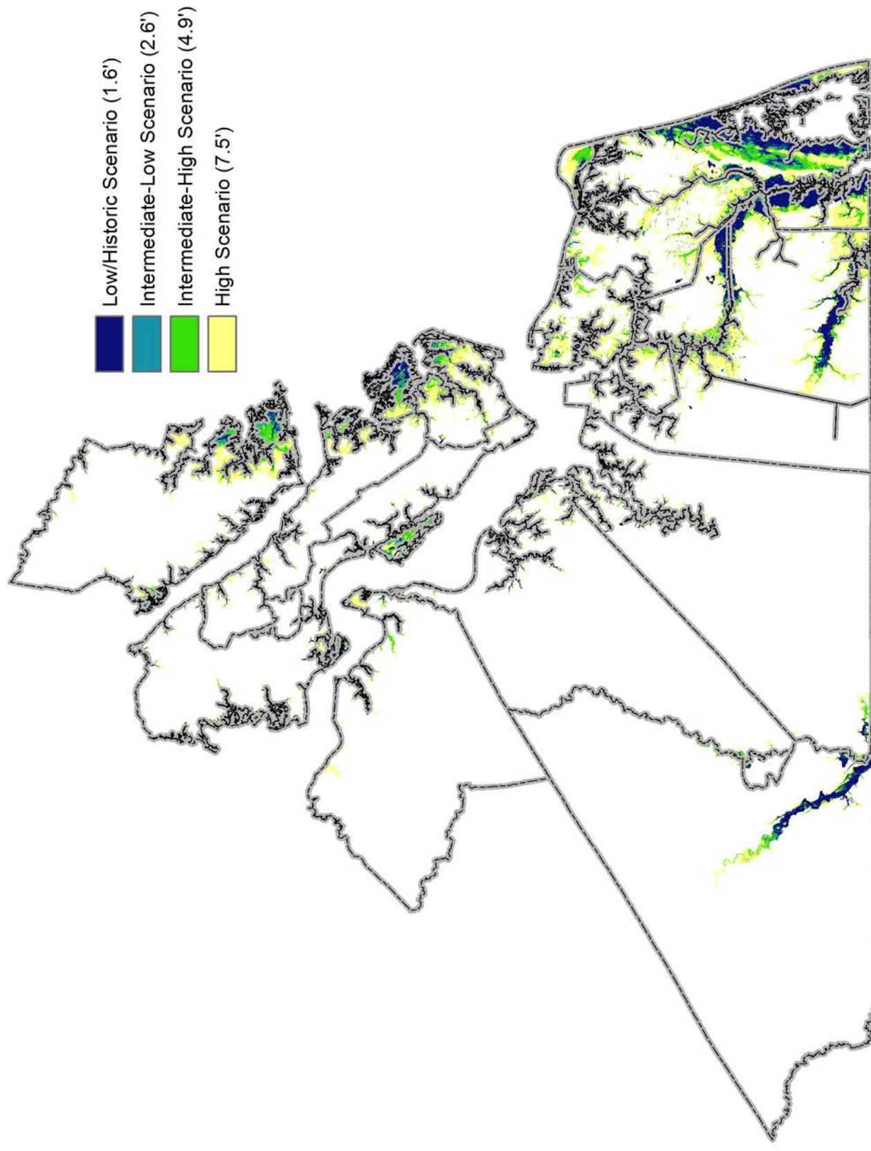
The final map showing areas potentially inundated at MHHW in 2100 under each sea level rise scenario.
