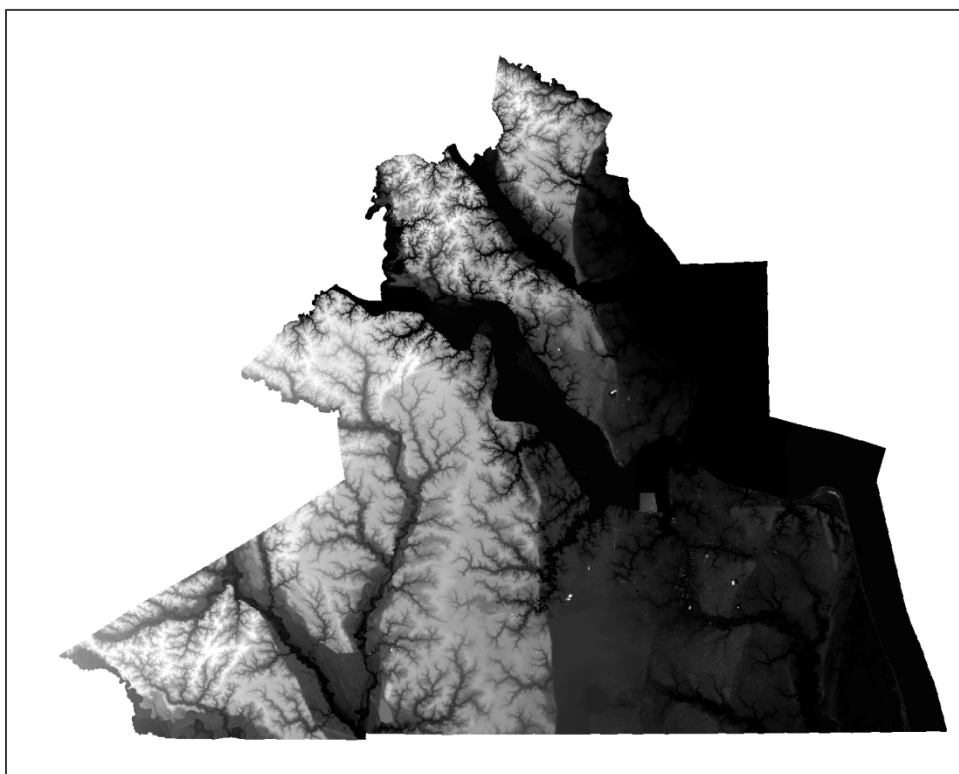
Step 1: Merging the regional DEM and MHHW surface.
