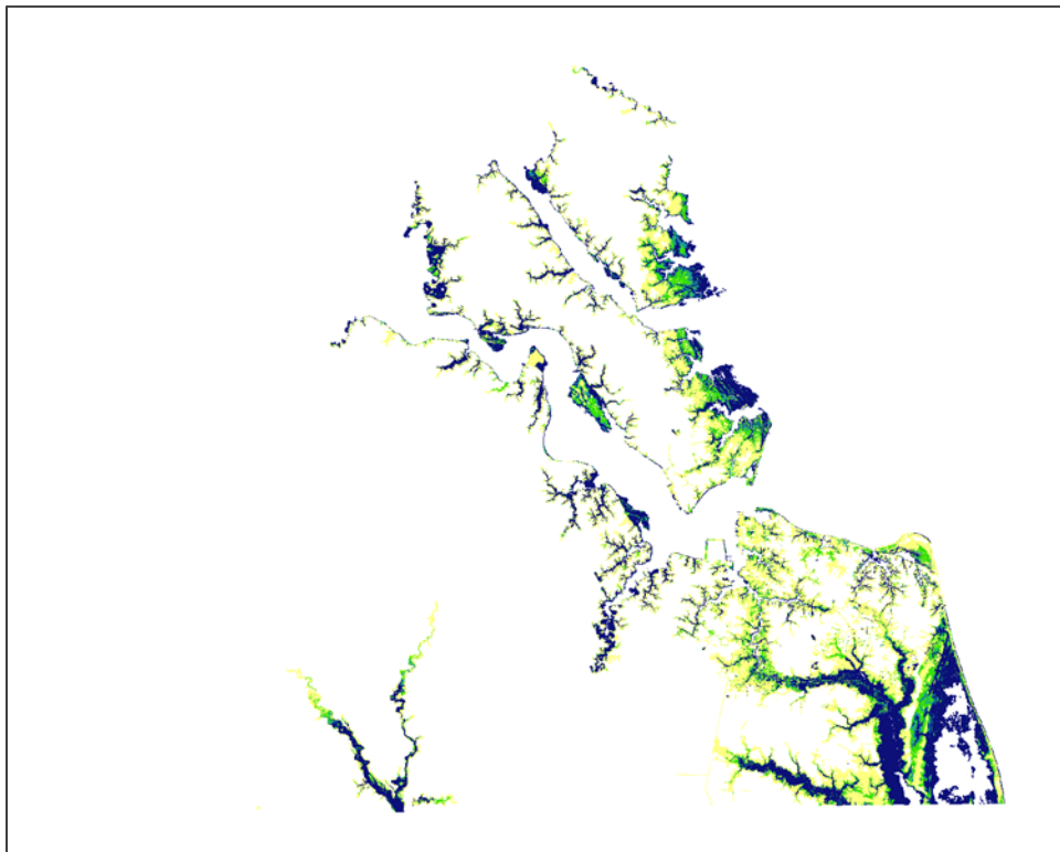
Step 7: Merging the four 2100 projection scenarios (1.6', 2.6', 4.9', and 7.6') to create a single raster for mapping.
