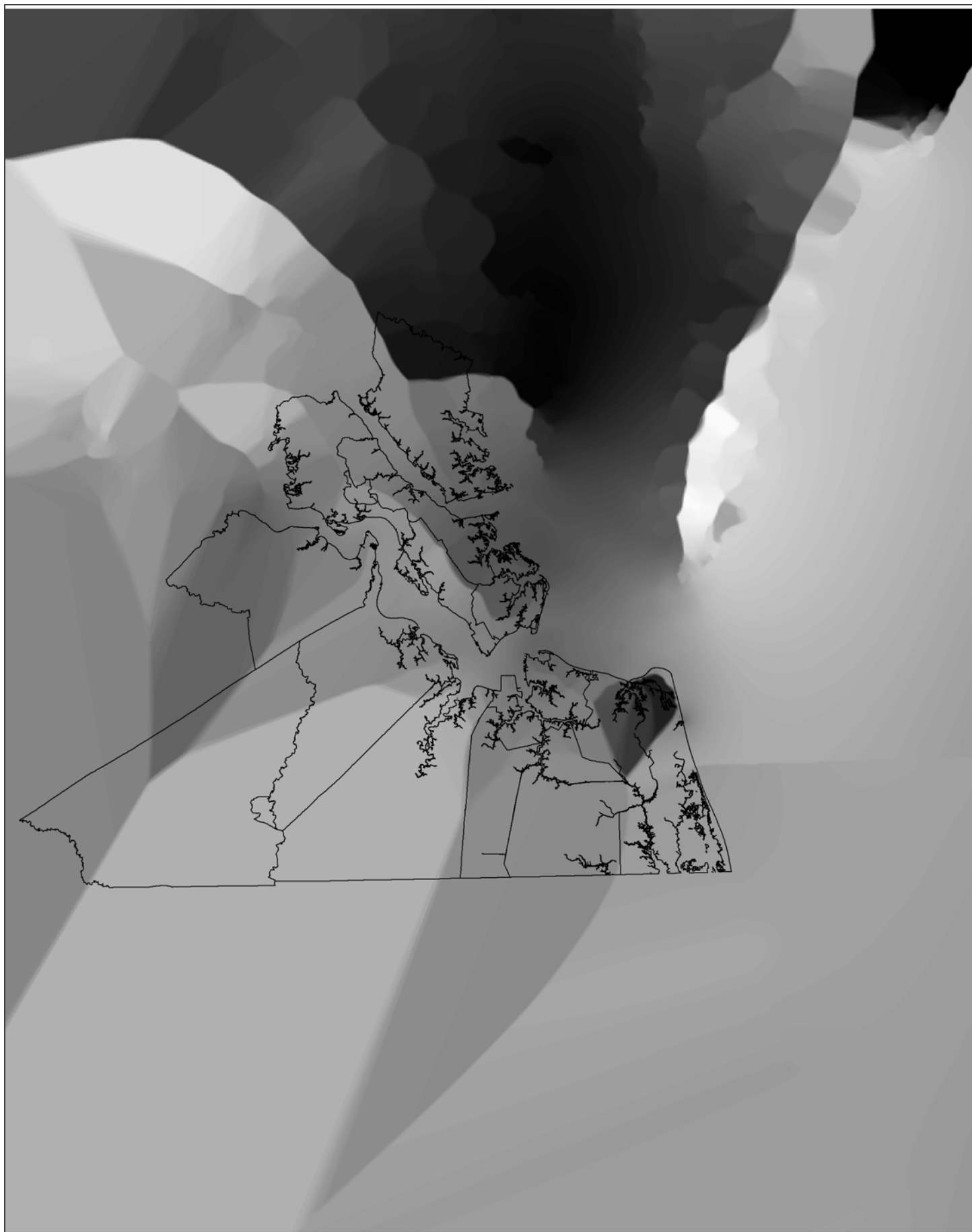
The regional Mean Higher High Water surface was created using Inverse Distance Weighting (IDW) Interpolation. The regional boundary is shown to illustrate scale.
