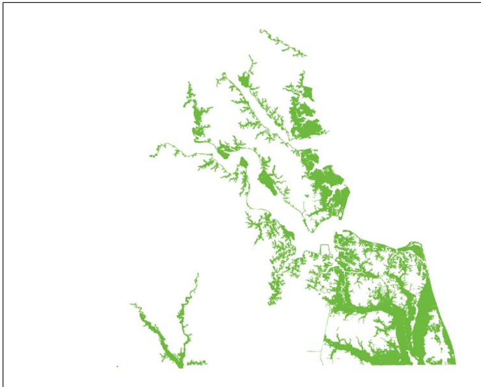
Step 6: Reclassifying the clipped raster to a single value.
