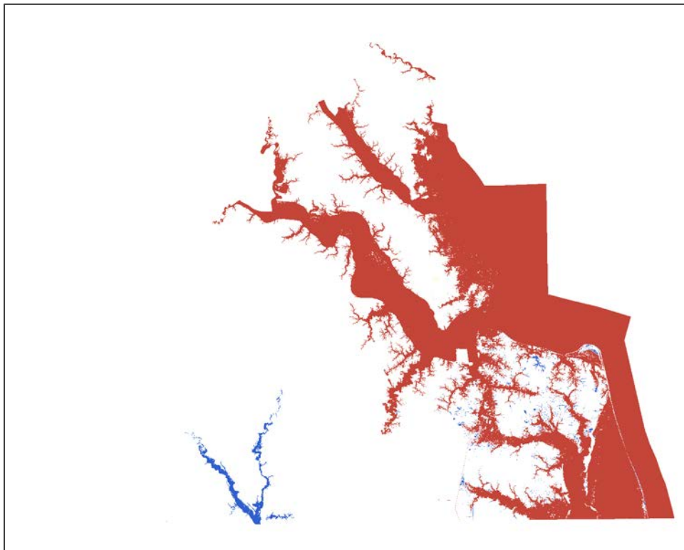
Step 3: Grouping the various hydrologically connect regions.
