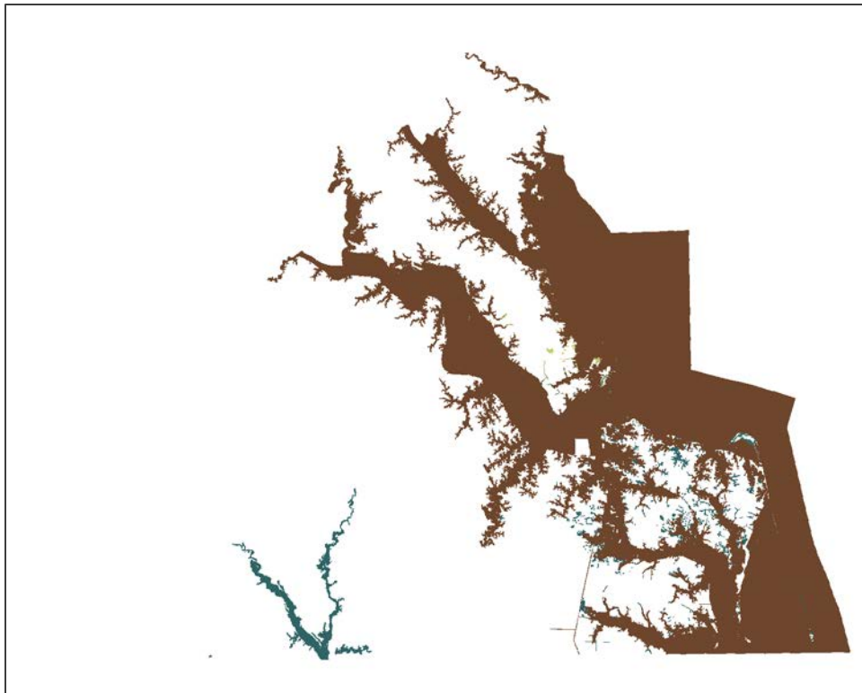
Step 4: Extracting significantly large hydrologically connected regions.
