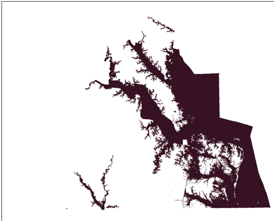
Step 2: Creating the single value raster. This shows all areas with a value of a less than 7.5 feet above MHHW (the highest scenario).
