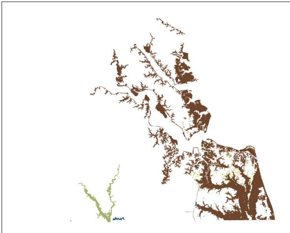
Step 5: Clipping the extracted raster to the original DEM's shoreline.
